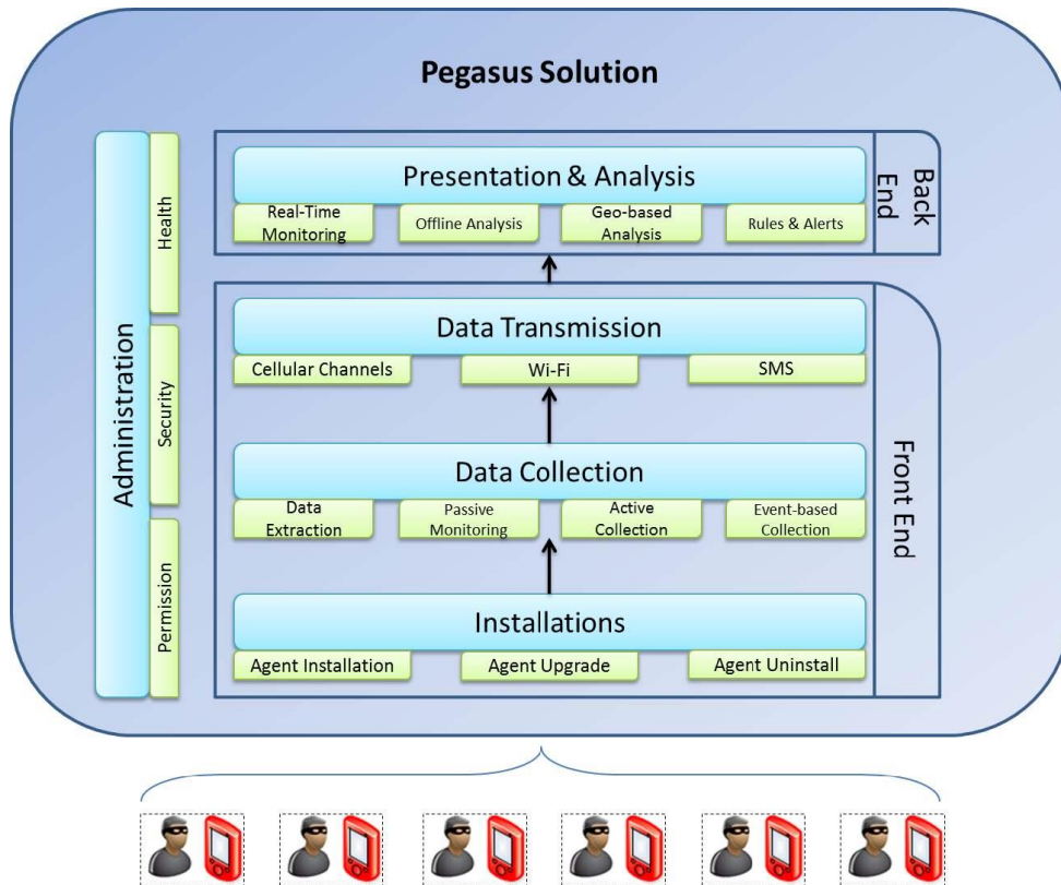
Figure 1: Pegasus High Level Architecture
