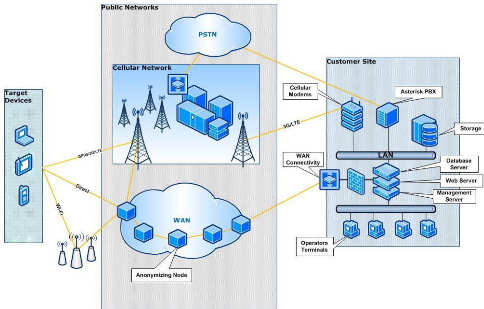
Figure 10: Solution Architecture
