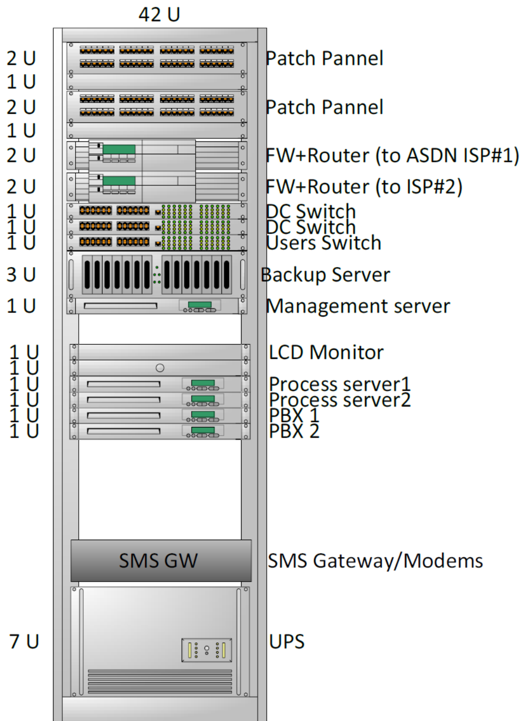
Figure 11: Pegasus Hardware
